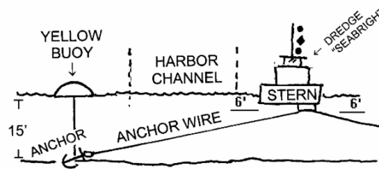
DREDGE "SEABRIGHT" -- LOOKING SOUTH TYPICAL MOORING CONFIGURATION (NOT TO SCALE)
